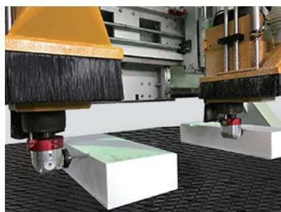
主軸旋轉C軸(義大利製) Spindle rotation axis (made in Italy)
